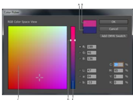
Color Picker
